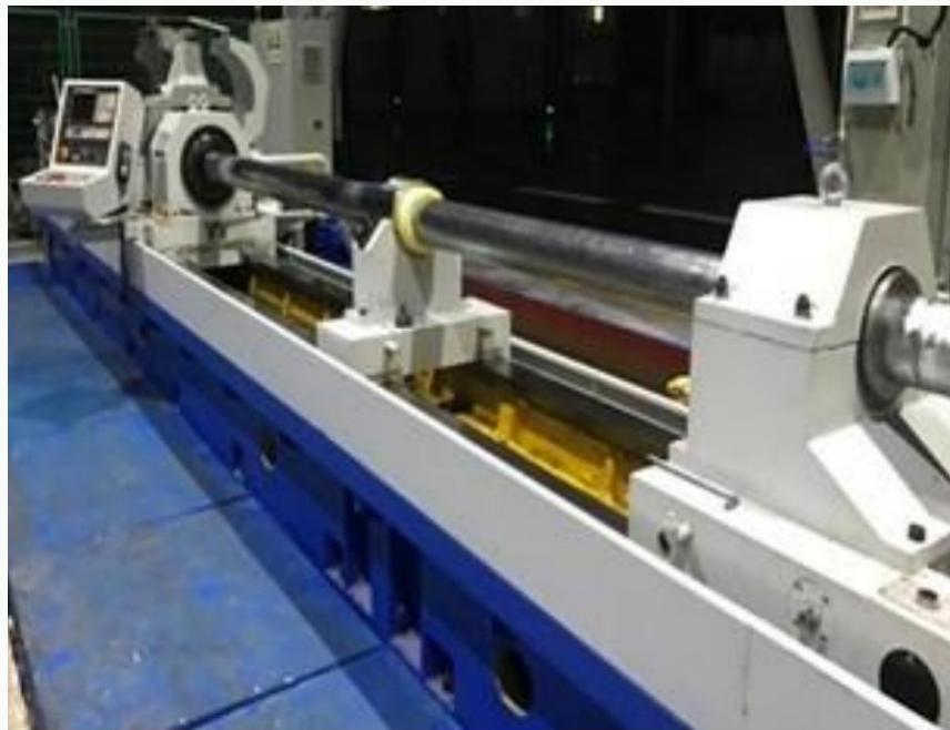
■ 3M Deep Hole Boring CNC Machine
