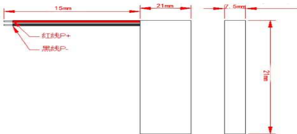
Battery
